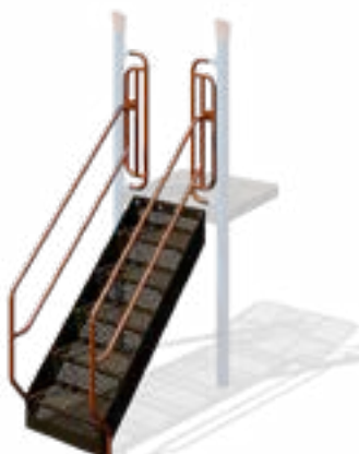
Ground-to-Deck Stairs Available for 3.5" and 5" posts 2', 3', 4', 5', 6', and 8' deck heights
